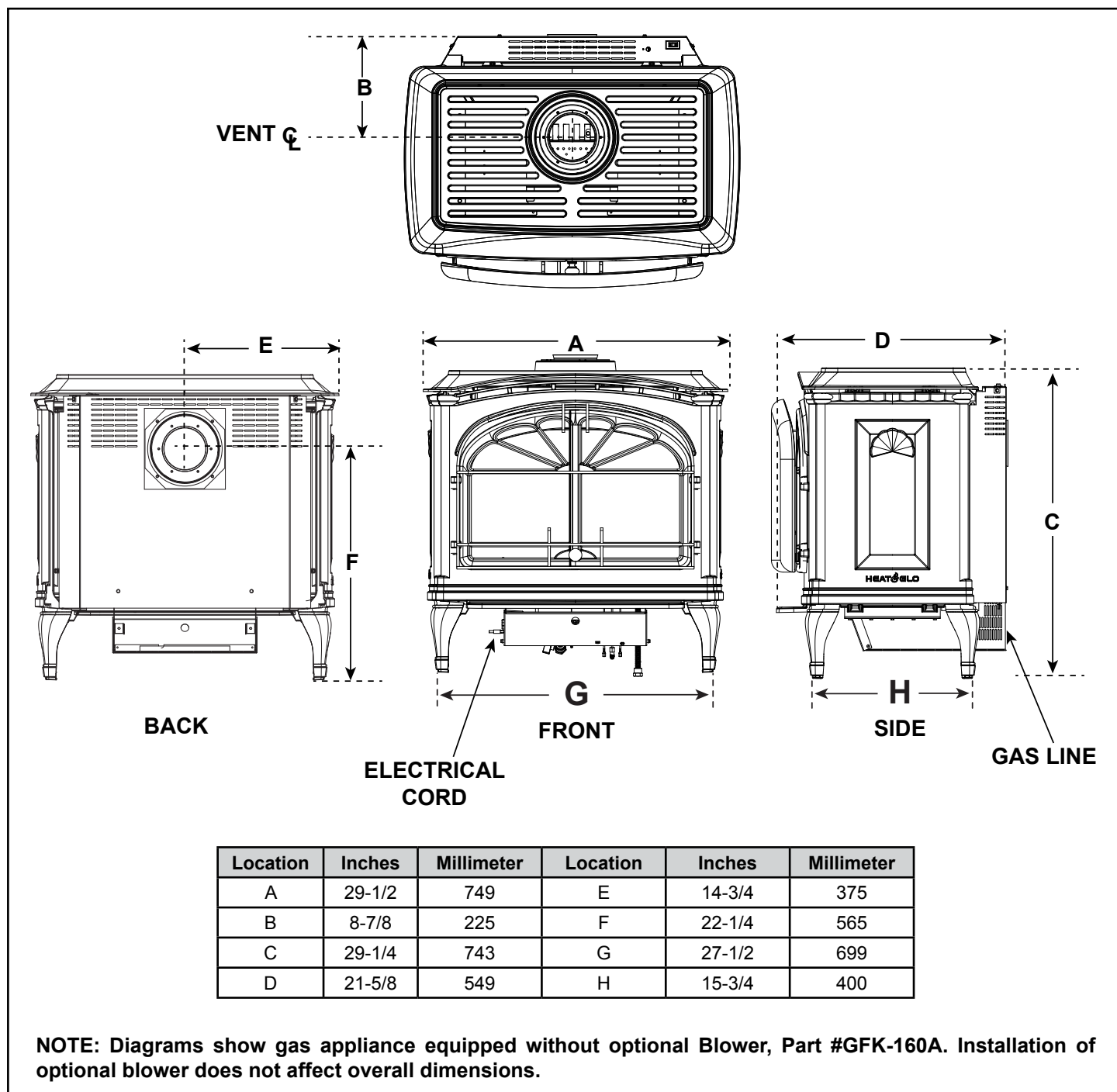
Figure 3.1 Appliance Dimensions
