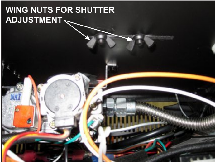
Figure 9.1 - Air Shutter
