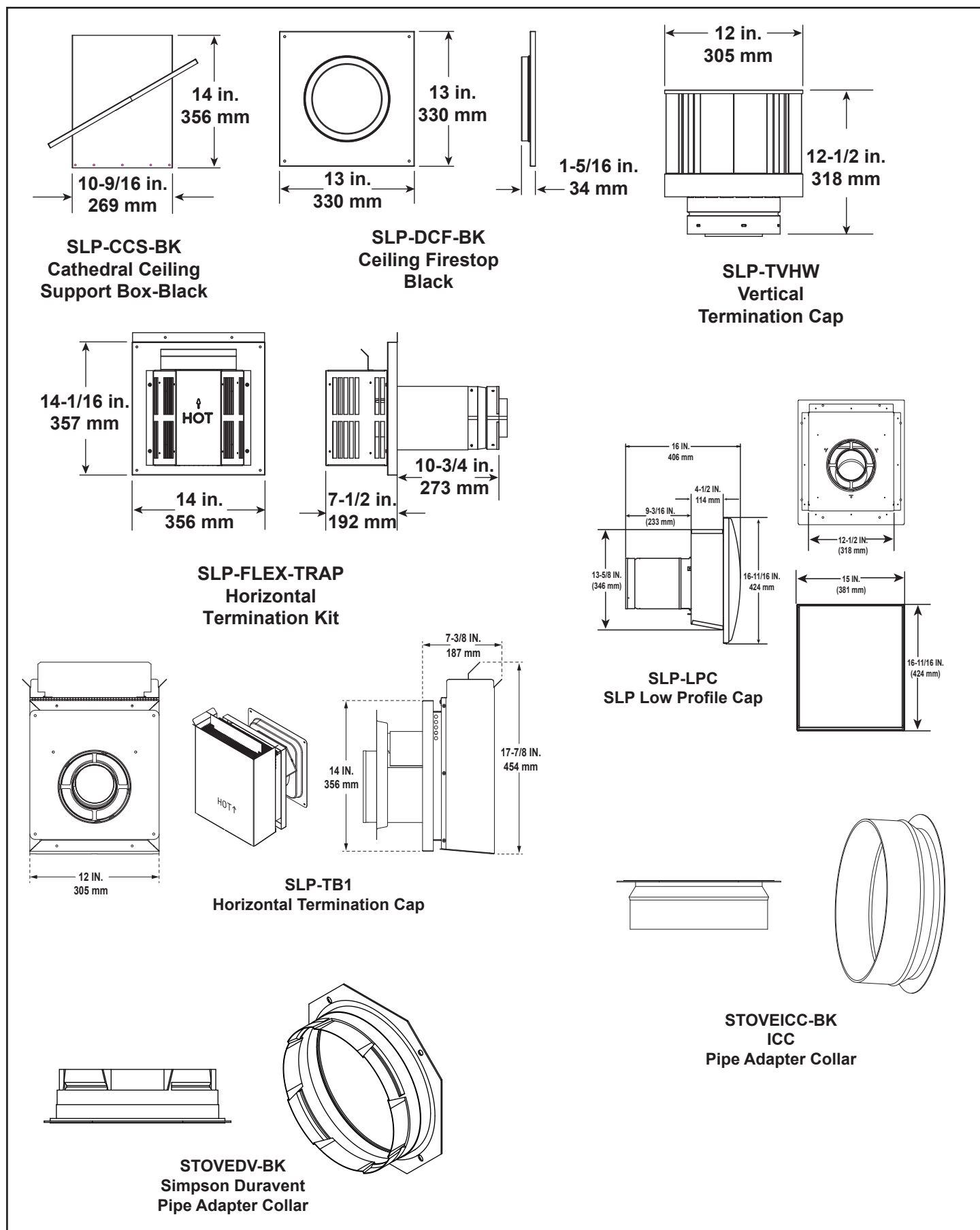
Figure 11.3 - SLP Series Vent Components
