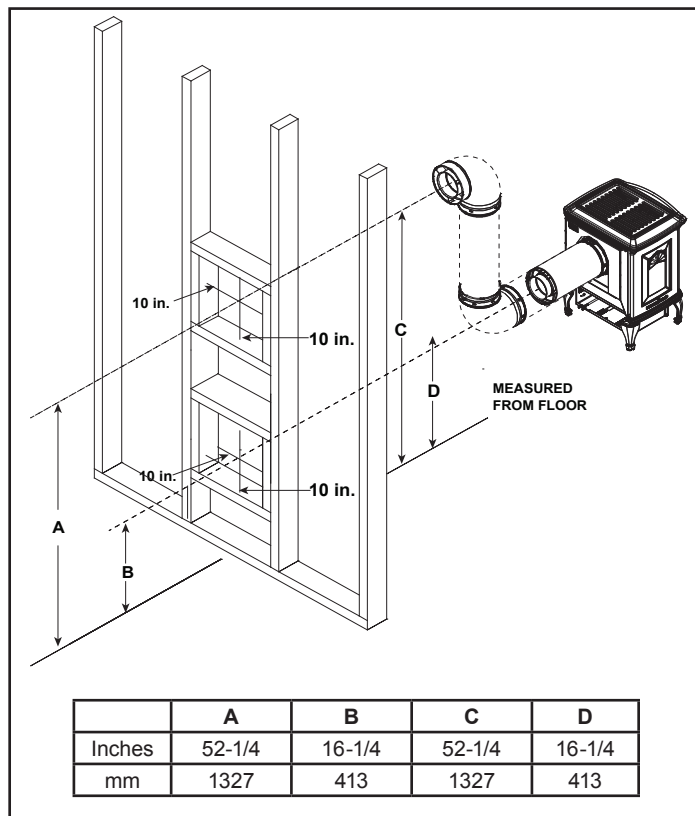
Figure 5.2 - Wall Penetration
