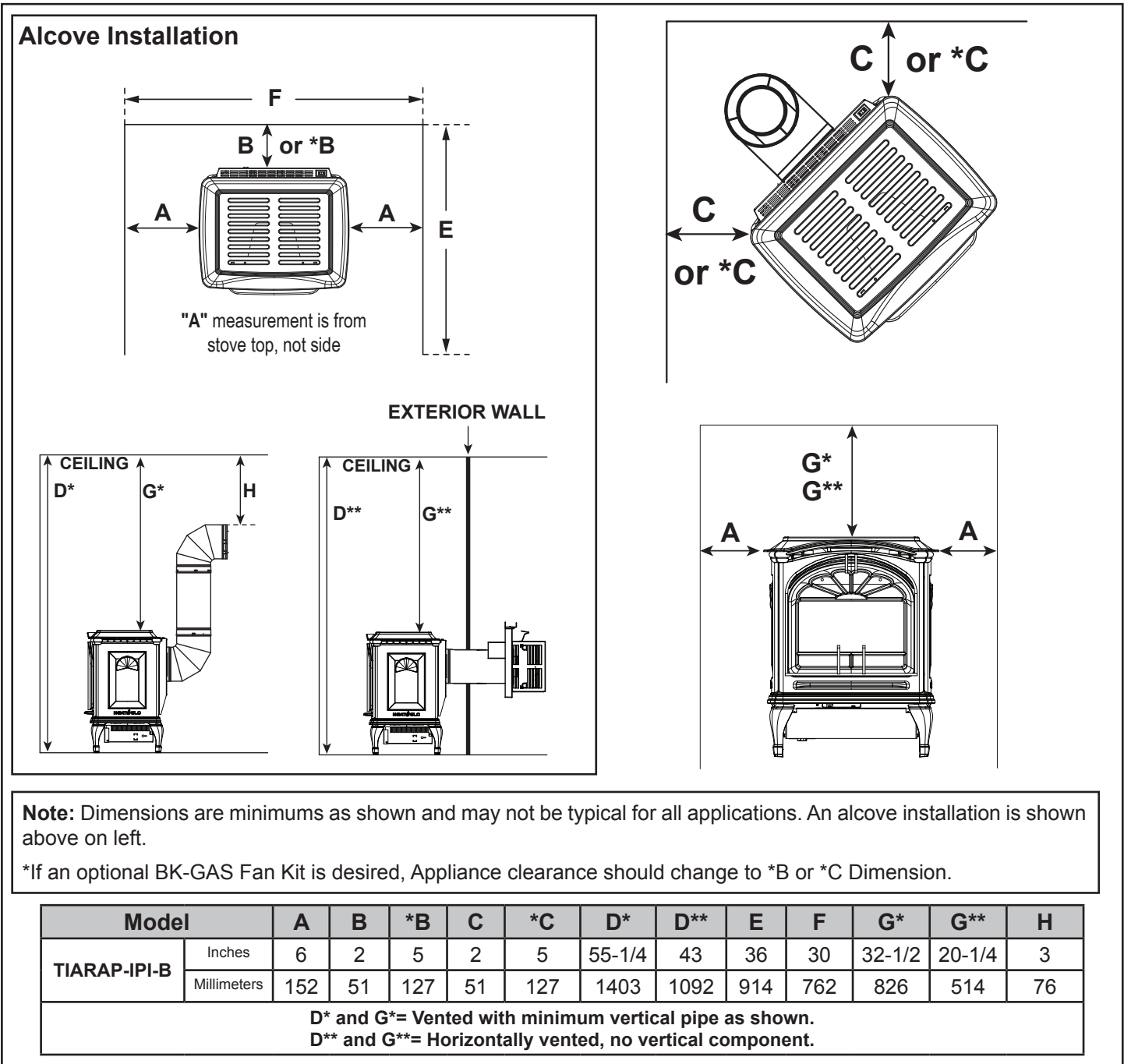
Figure 3.2 - Appliance Locations
