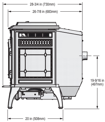
Figure 9.1 -Side View
