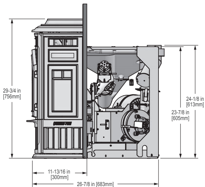
Figure 8.6 - Side View with Basic Surround Set
