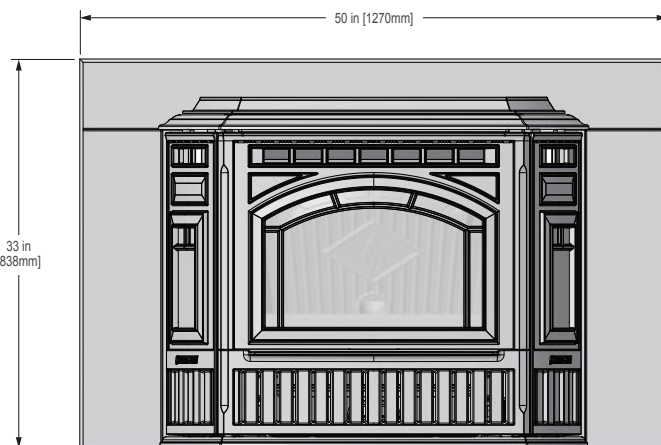
Figure 8.5 - Front View with Basic Surround Panel Set
