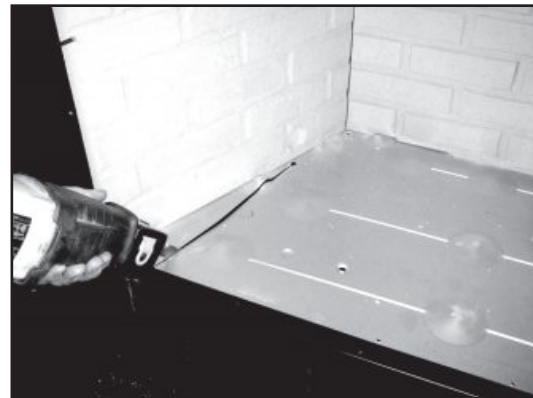
Figure 11.3 - Using a saws-all, cut out the floor.
