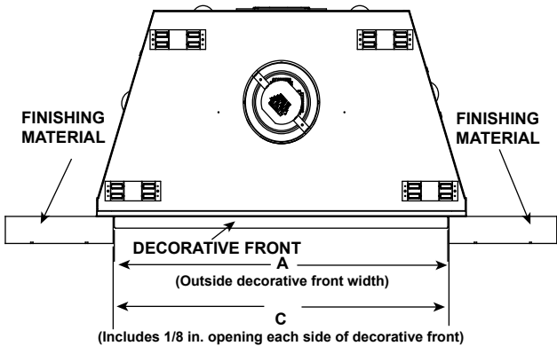
Figure 10.7 Finishing Material Thickness Greater Than One Inch
