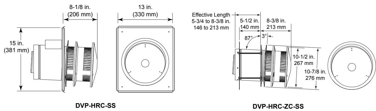
Figure 12.5 DVP Vent Components
