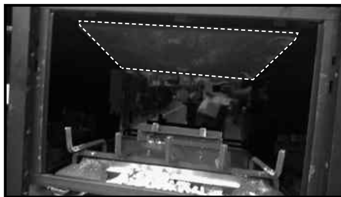
Figure 4. Install Top Refractory Panel
